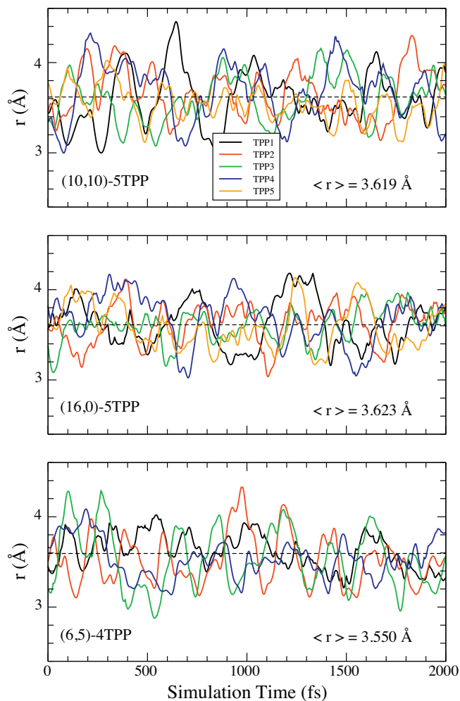
Figure 5. Adsorption distance r as a function of time for the molecular dynamic simulation of the CNT-TPP compounds at 373 K. The dashed lines indicate the average adsorption distance. The different curves indicate the evolution of r for each TPP molecules.
