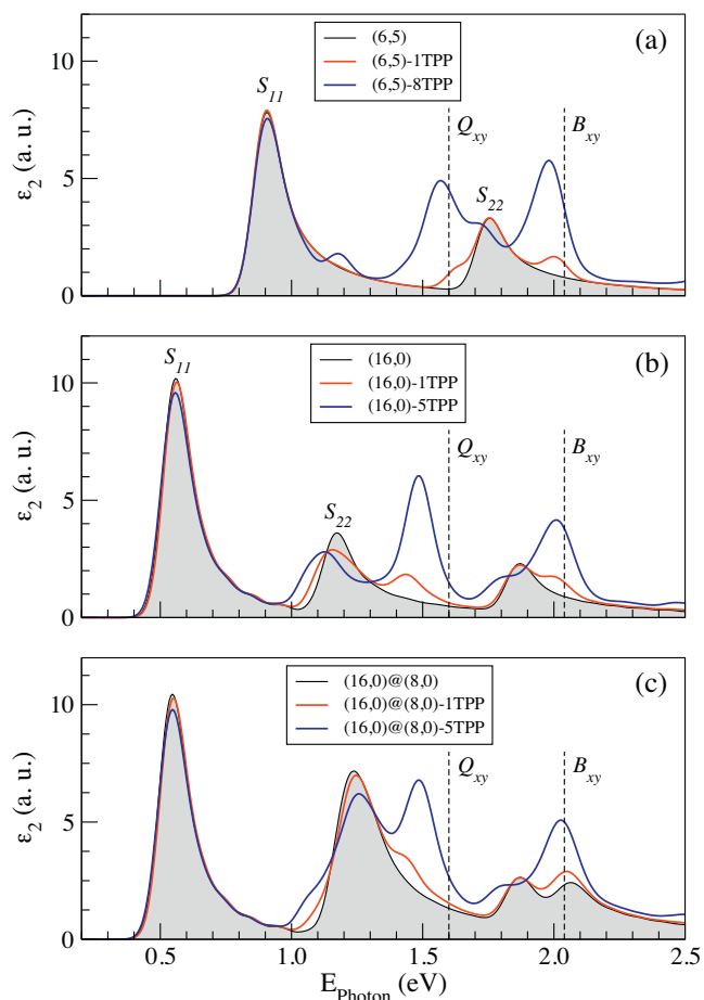
Figure 4. Imaginary part of the dielectric function for the semiconducting CNT-TPP compounds: (a) the (6,5)-TPP, (b) the (16,0)-TPP, and (c) the (16,0)@(8,0)-TPP. The dashed lines indicate the Q_{xy} and B_{xy} absorption bands of the free TPP molecule.
