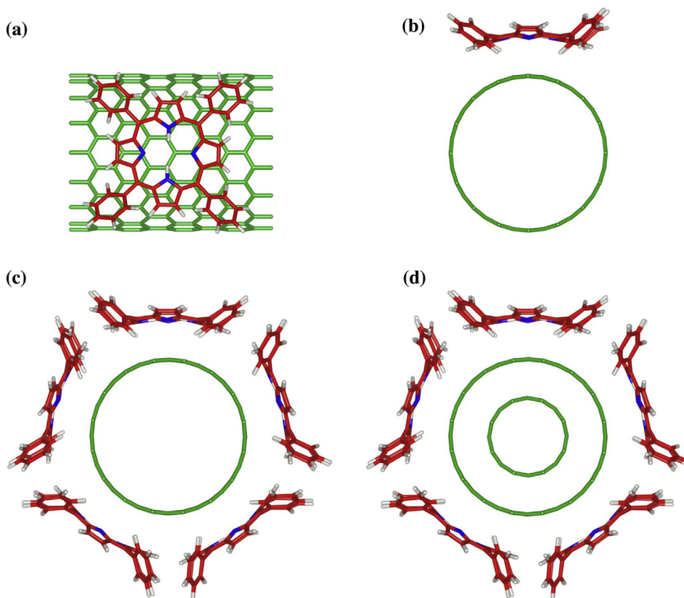
Figure 2. Schematic representation of TPP molecules adsorbed on single- and double-wall CNTs in the equilibrium geometry. (a)–(b) Top and front views of (16,0)-1TPP, (c) (16,0)-5TPP, and (d) (16,0)@(8,0)-5TPP.
