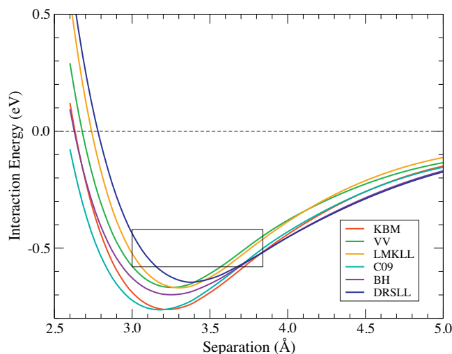
Figure 1. Interaction energy as a function of the separation for the benzene adsorption on graphene calculated with different parametrizations for the Van der Waals density functional. The square box indicates the available experimental data.
