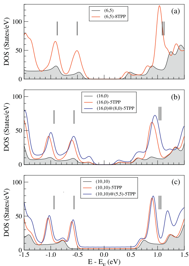
Figure 3. Density of states for the CNT-TPP compounds: (a) (6,5)-8TPP, (b) (16,0)-5TPP and (16,0)@(8,0)-5TPP, and (c) (10,10)-5TPP and (10,10)@(5,5)-5TPP. The vertical lines represent the frontier orbitals of the free TPP molecule.
