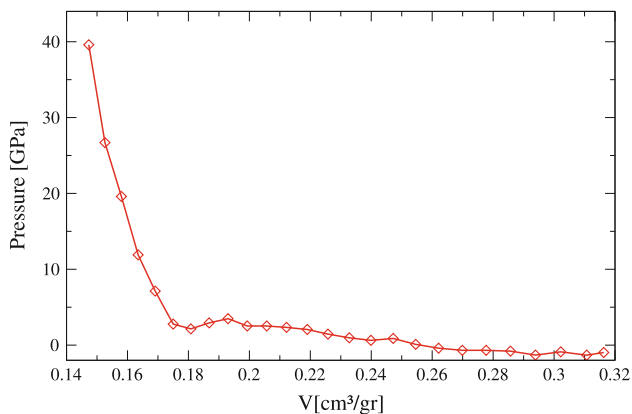
Fig. 2 P – V equation of state of amorphous GeO 2
